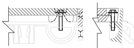
FRAME & COVER SHOWING DEBRIS CHUTE
