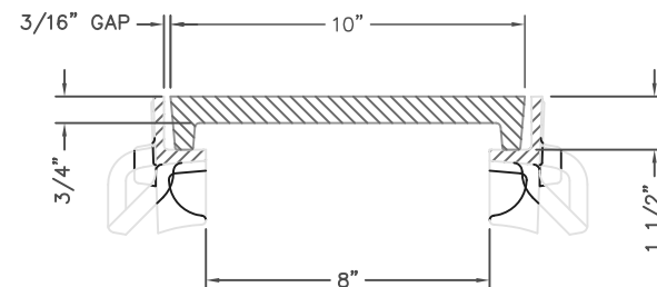
R-4999-BX TYPICAL SECTION TYPE "D" LID w/ TYPE "B" FRAME
